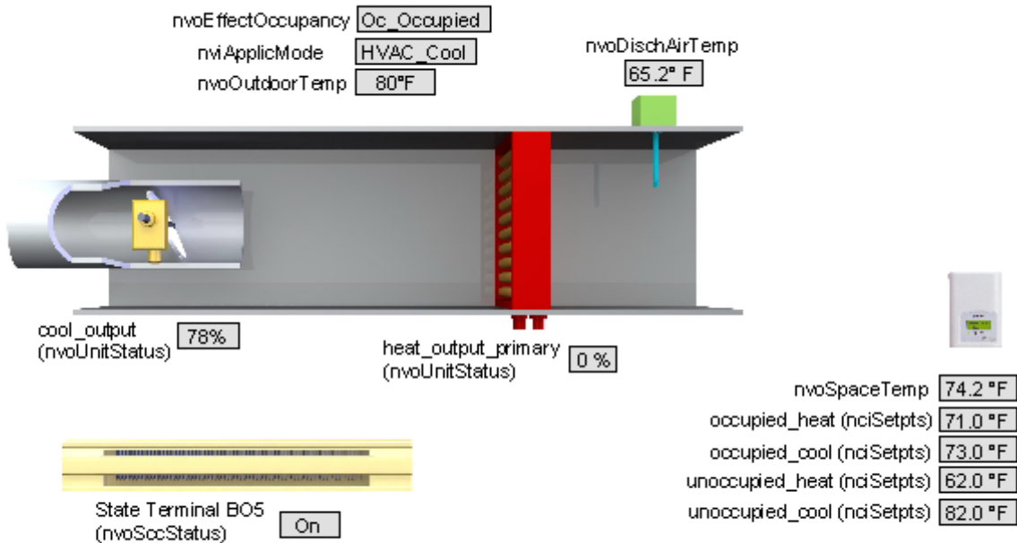
Graphical User Interface (GUI) example of a zoning thermostat
