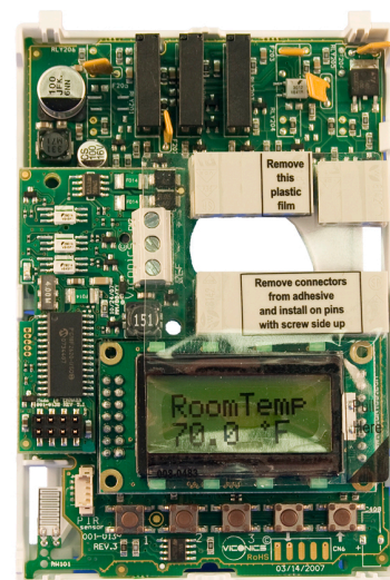
Terminal Equipment Controller assembly (VT300F5000B shown)
