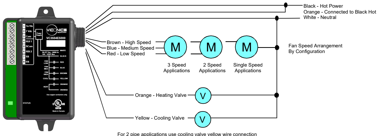
VC3504E Relay Pack
